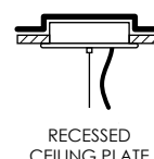
RECESSED CEILING PLATE CUT OUT Ø102mm
